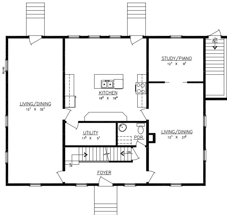
MAIN FLOOR AREA = 1525 S.F.
